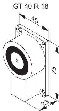
Tür-Haftmagnet, Haltekraft: 300 N magnetic clamp for fire door, hold-on power: 300 N
