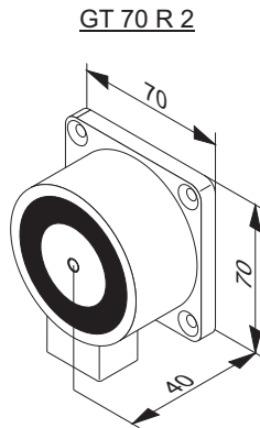
GT 70 R 2 Tür-Haftmagnet, Haltekraft: 1372 N magnetic clamp for fire door, hold-on power 1372 N
